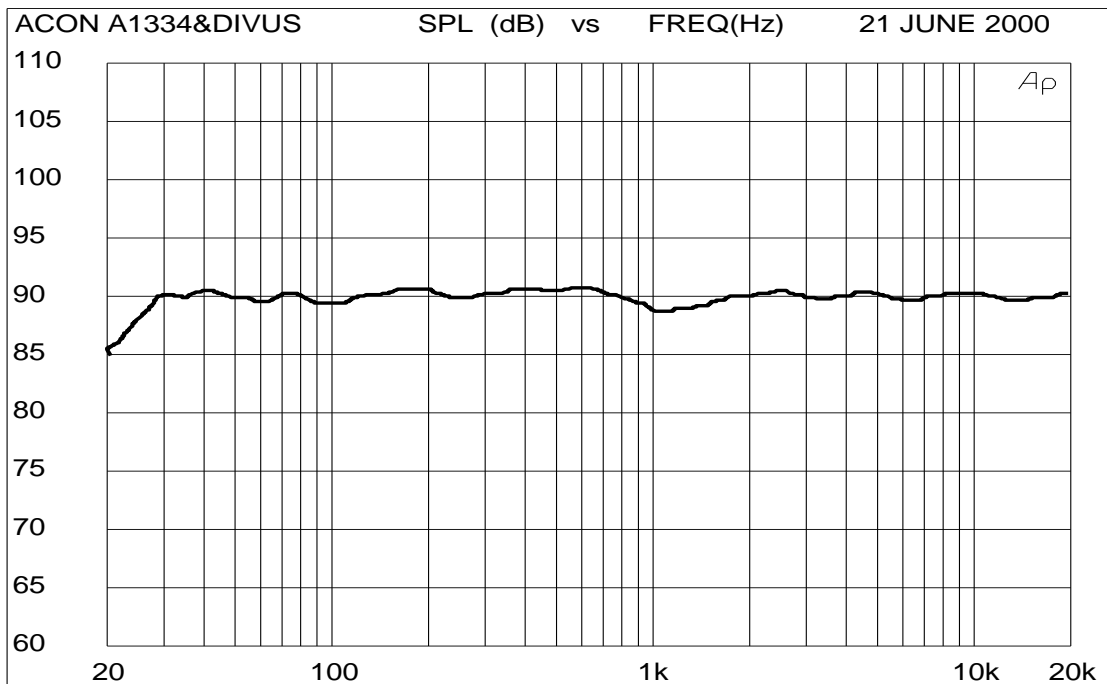
Obr. 9b: Active speaker ACON A1334/DIVUS frequency response, 1m on axis in studio conditions
